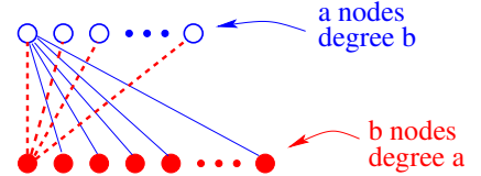
FIG. 2: The complete bipartite graph K_{a,b} .
