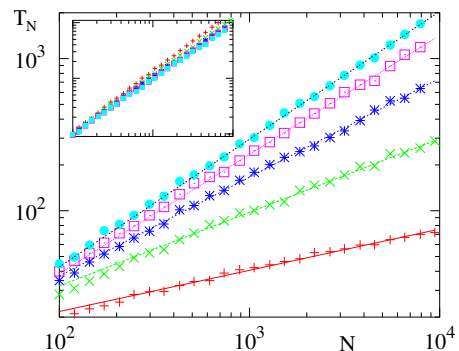
FIG. 4: Consensus time T_N versus N for the configuration model with degree distribution n_k = k^{-\nu} for \nu = 2.1 (+), 2.3 ( \times ), 2.5 (*), 2.7 ( \circ ) and 2.9 ( \bullet ). Data are based on 100 graph realizations and 10 realizations of VM dynamics on each graph. Lines represent the prediction (15). The inset shows the same data plotted in the scaled form \mu_2 T_N / \mu_1^2 versus N .
