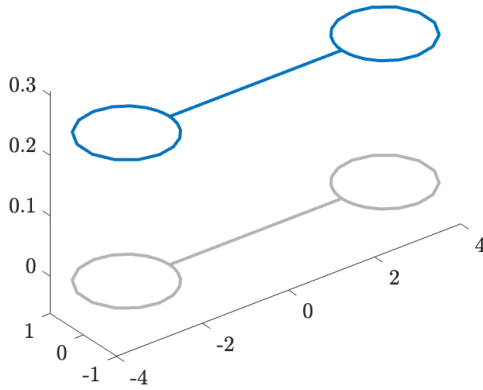
Eigenfunction 3, \lambda = -0.430
