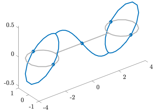
Eigenfunction 4, \lambda = -0.897
