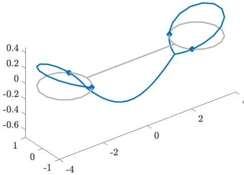
Eigenfunction 3, \lambda = -0.430
