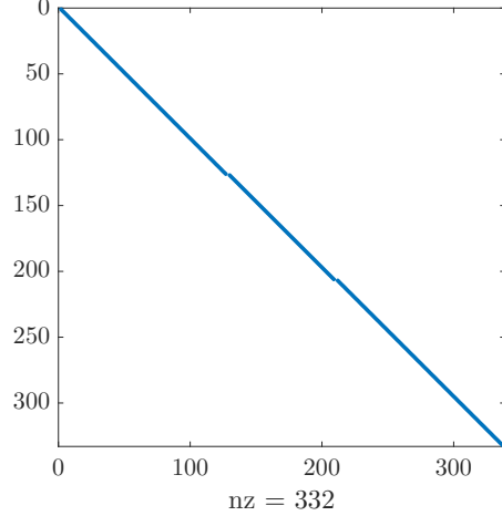
Interpolation Matrix–Uniform discretization
