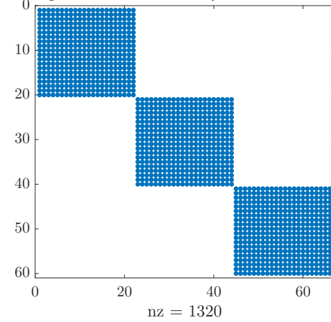
Interpolation Matrix–Chebyshev discretization
